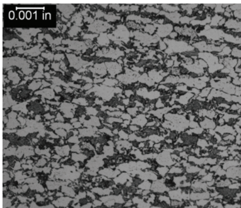
Microstructure showing exposure to intercritical temperatures, consisting of transformed pearlite in a ferrite matrix with a few grain boundary voids scattered throughout.
