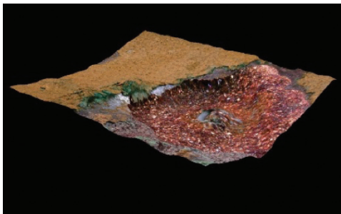
Two- and three-dimensional images of a copper heat exchanger tube that has been damaged from under-deposit corrosion (UDC).
